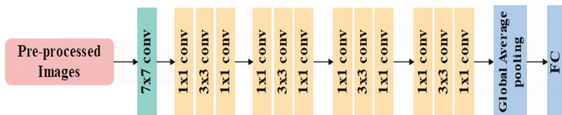
Figure 3. ResNet-50 Architecture.
