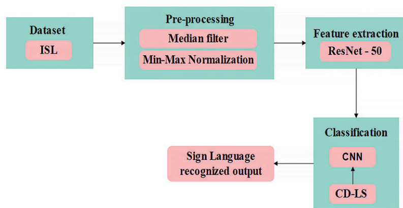
Figure 1. Process of Indian Sign Language Recognition.
