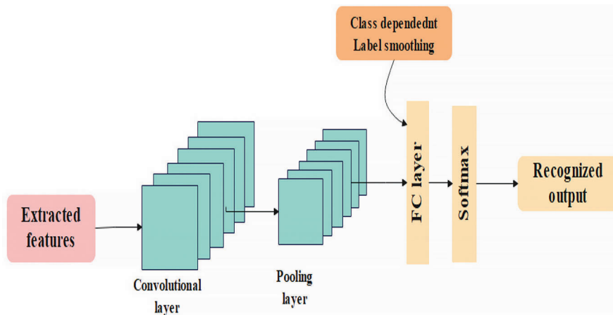
Figure 4. Architecture of CNN with CD-LS.
