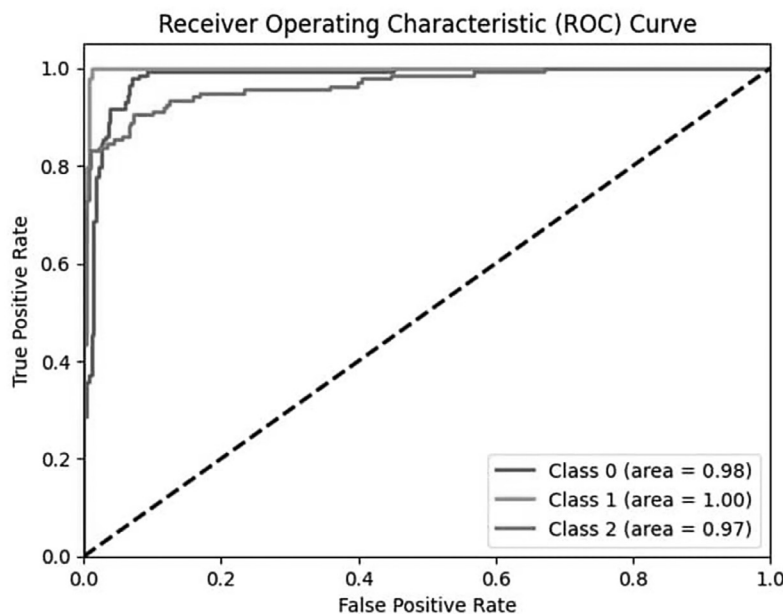
Figure 3. ROC curve area for proposed method.
