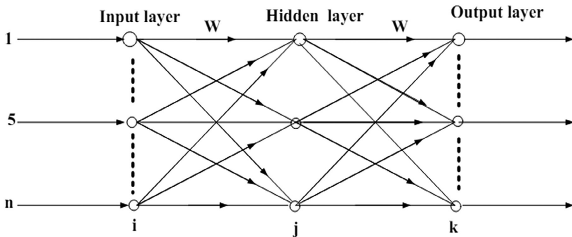
Figure 2. Structure of Back Propagation.
