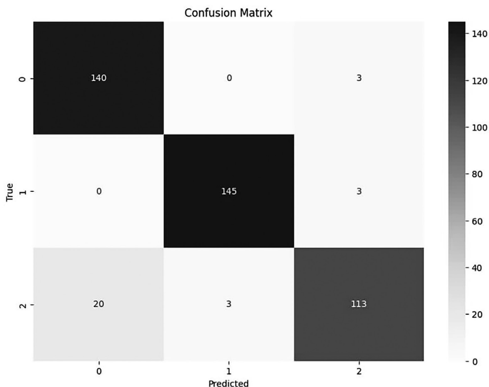
Figure 4. Confusion matrix for proposed method.
