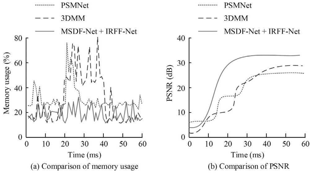
Figure 9. Overall performance comparison of the end-to-end network.
