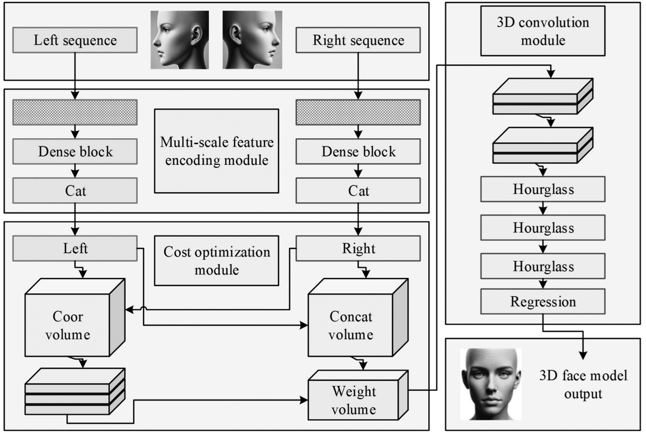
Figure 3. Schematic diagram of MSDF-Net network structure.
