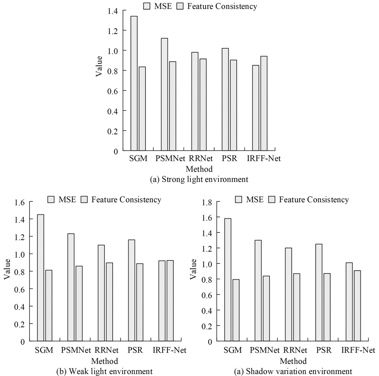
Figure 8. Robustness test under illumination variation.
