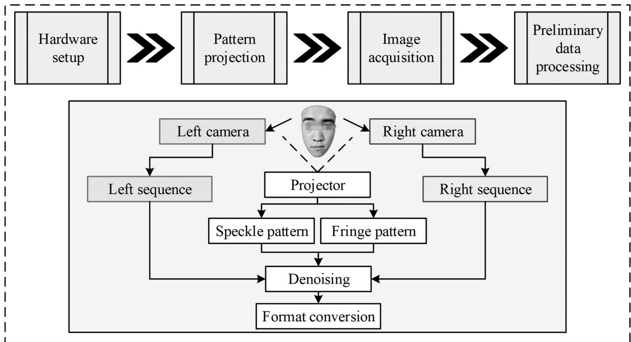
Figure 2. Detailed process of data acquisition.
