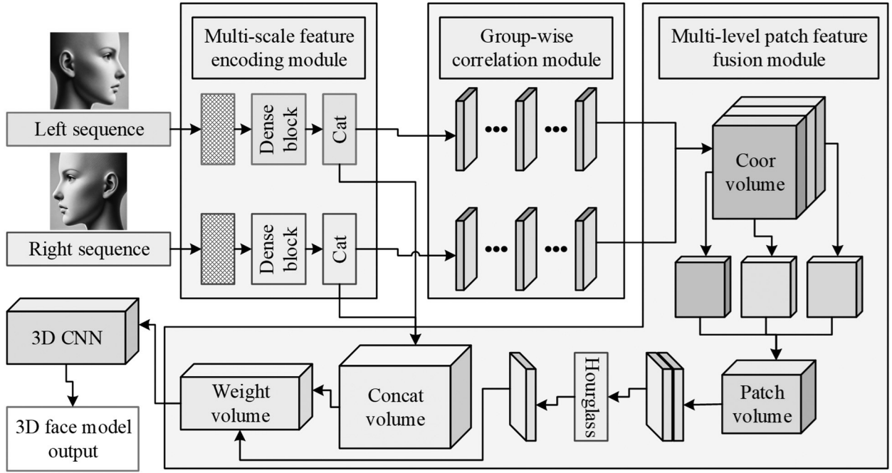
Figure 4. Schematic diagram of IRFF-Net network structure.
