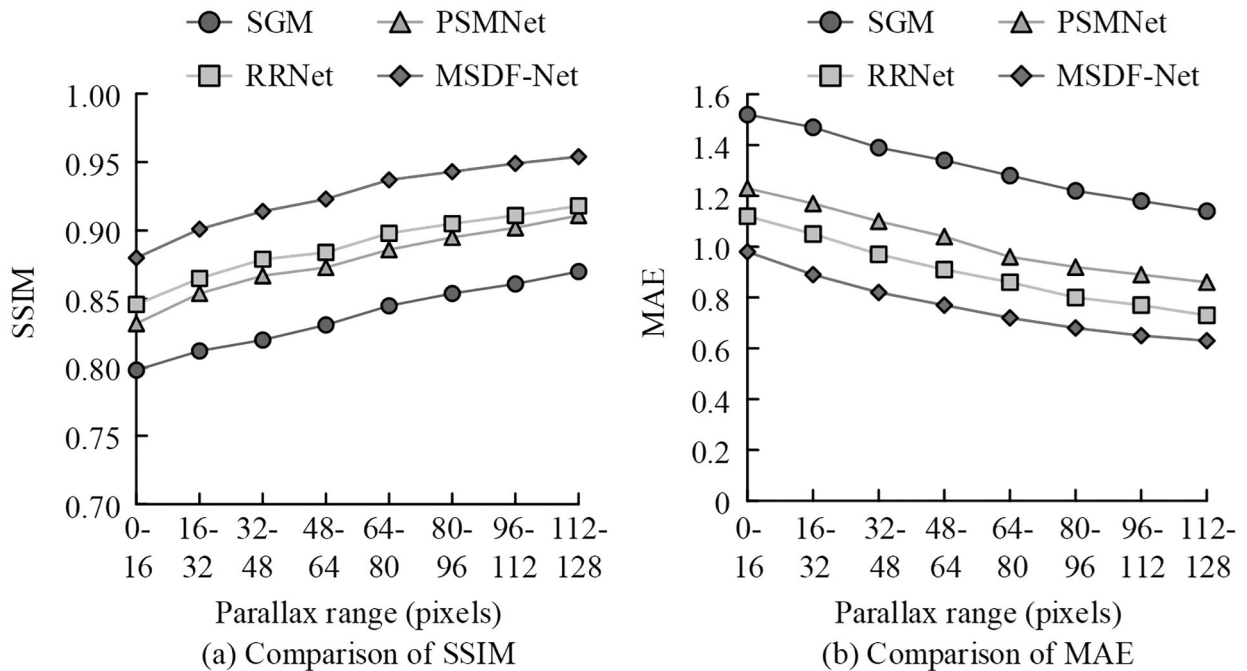
Figure 7. Performance verification results of MSDF-Net.
