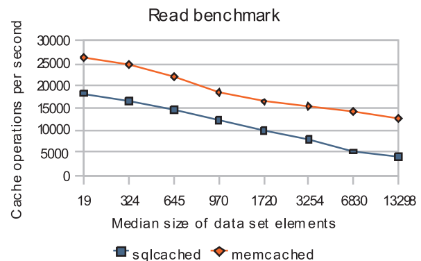
Figure 1. Results of simple key-value read benchmarks.
